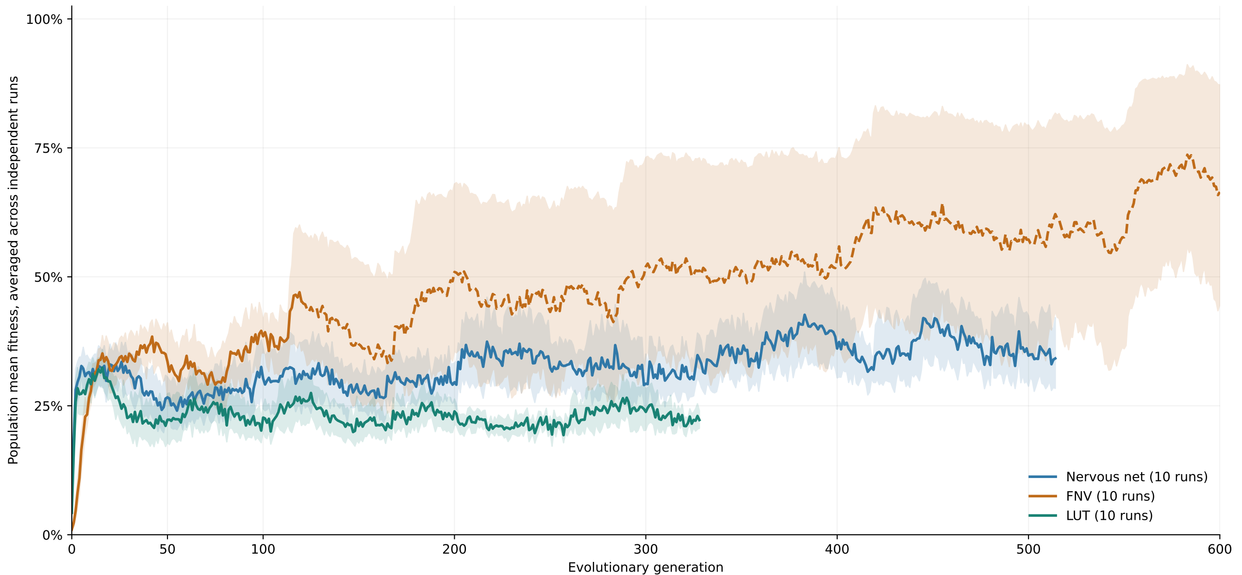
Fig. 18. A-count parity queried by B: developmental evolution through generation 600.
