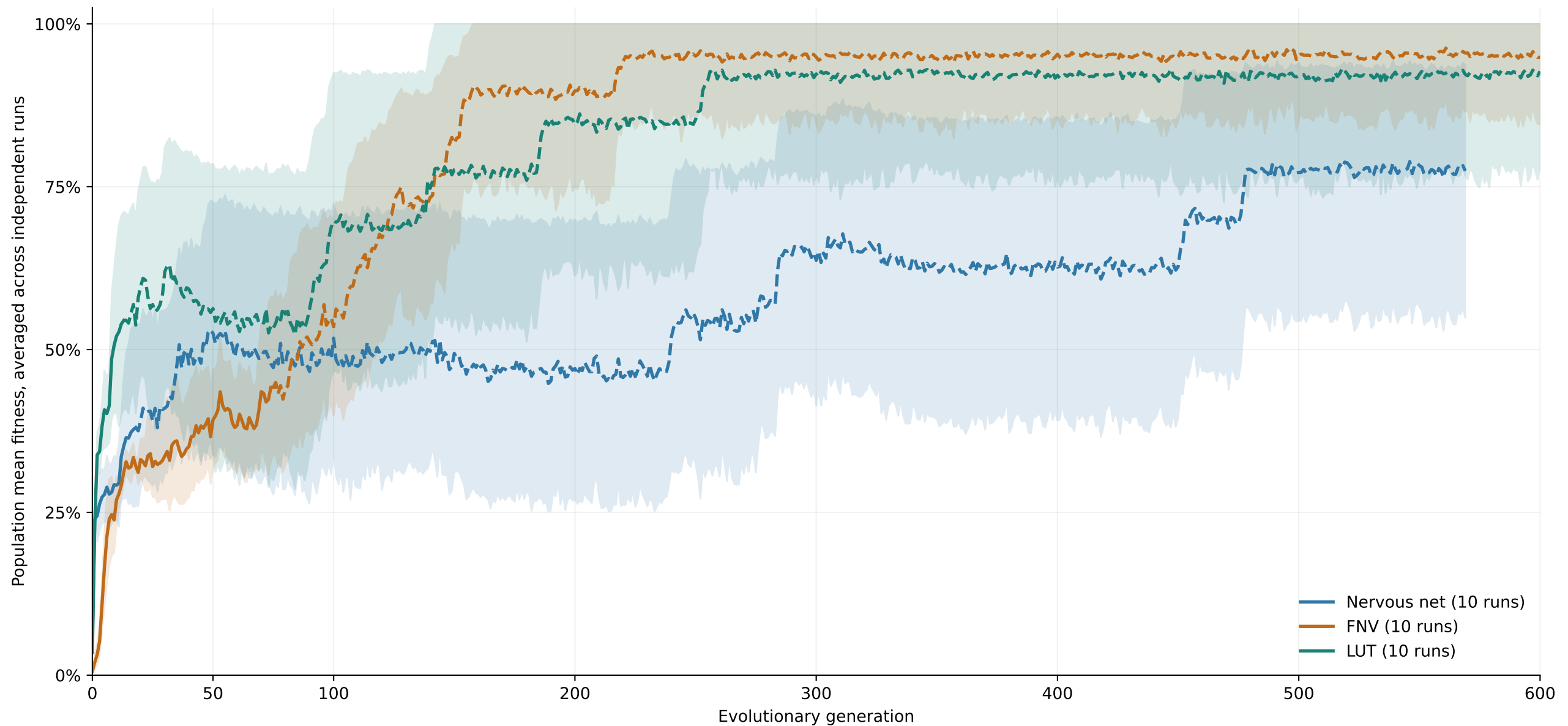
Fig. 21. Burst x3: developmental evolution through generation 600.
