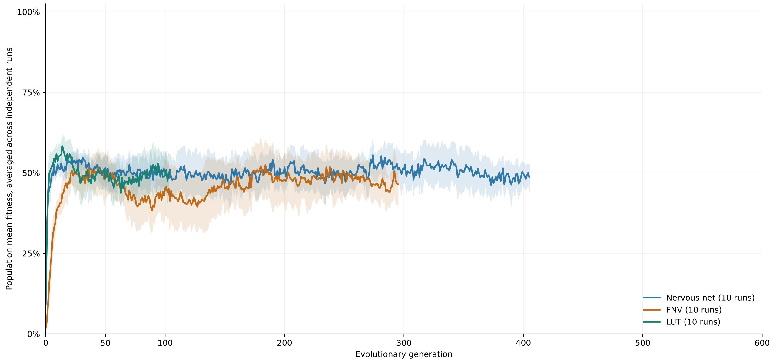
Fig. 24. Collision serializer (2-to-1): developmental evolution through generation 600.
