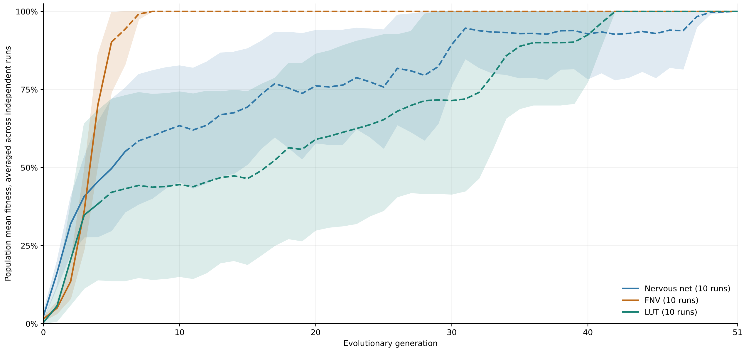
Fig. 5. Echo (delay 3): developmental evolution through generation 51.
