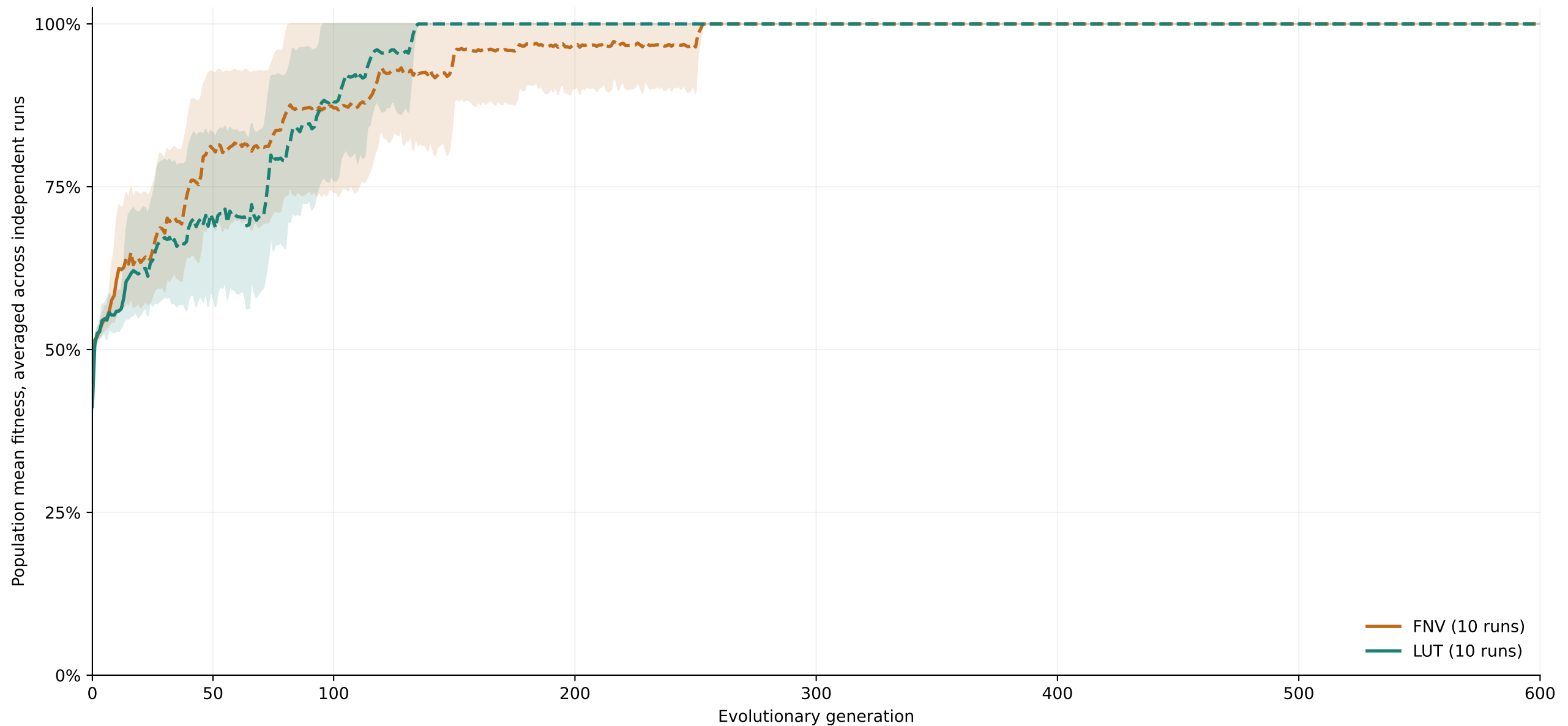
Fig. 31. Half adder: developmental evolution through generation 600.
