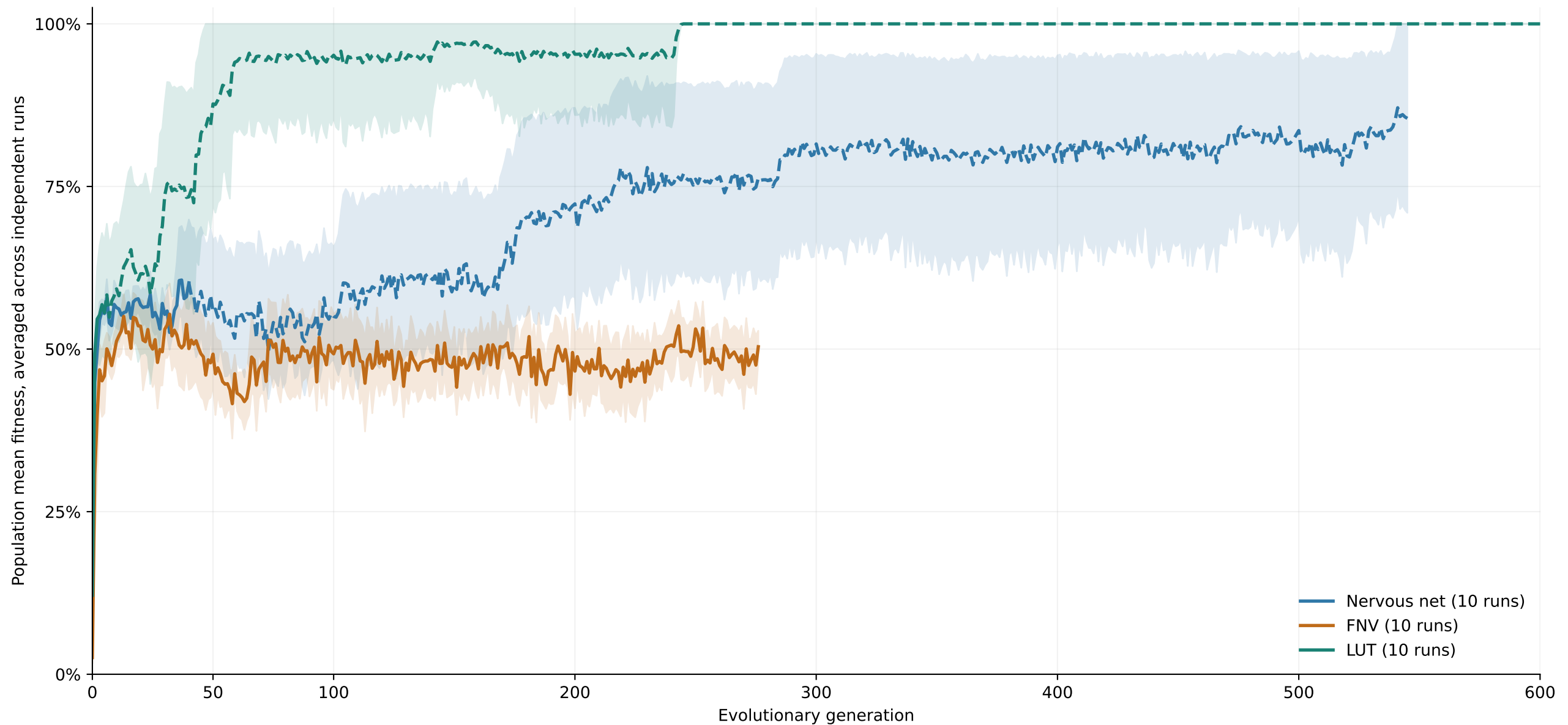
Fig. 33. Majority-3 (temporal): developmental evolution through generation 600.
