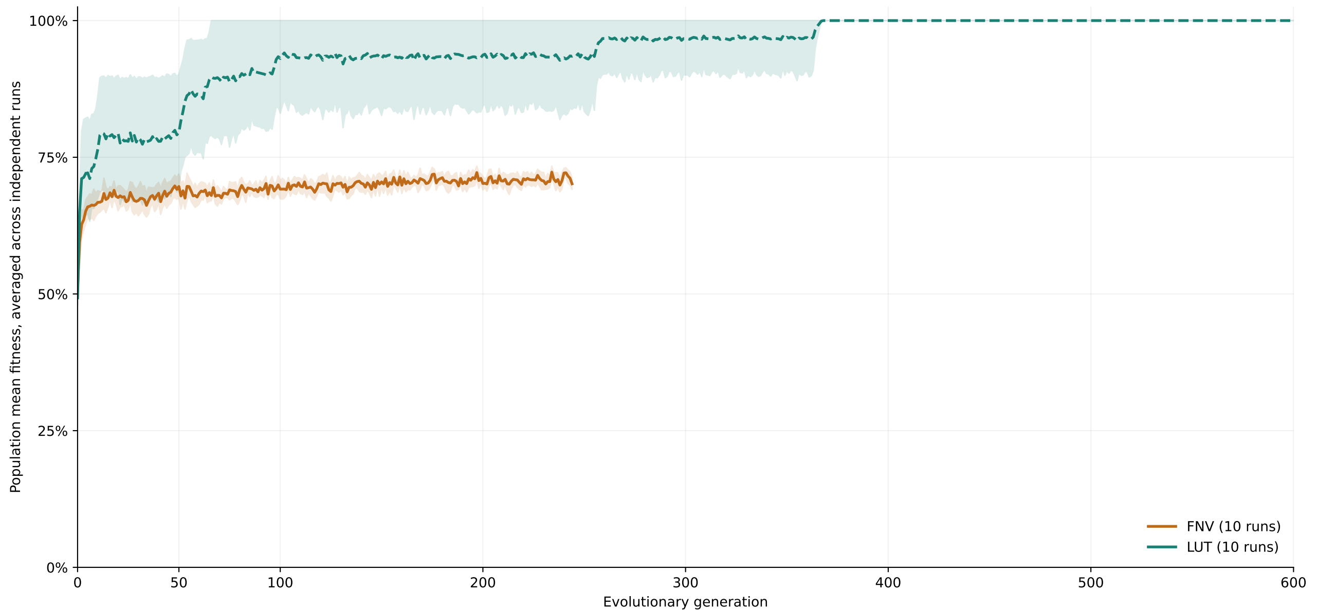
Fig. 32. Majority-3: developmental evolution through generation 600.
