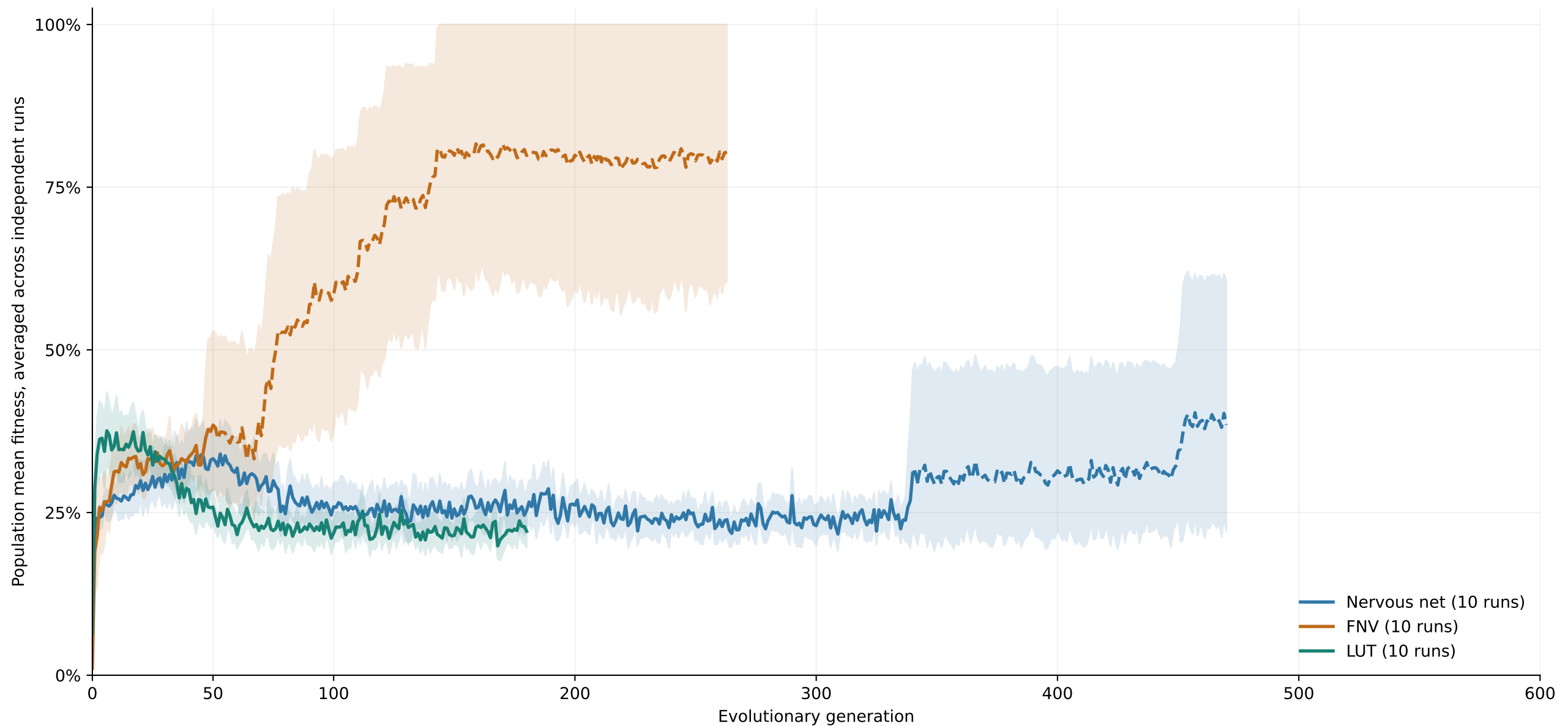
Fig. 37. NOR (temporal): developmental evolution through generation 600.
