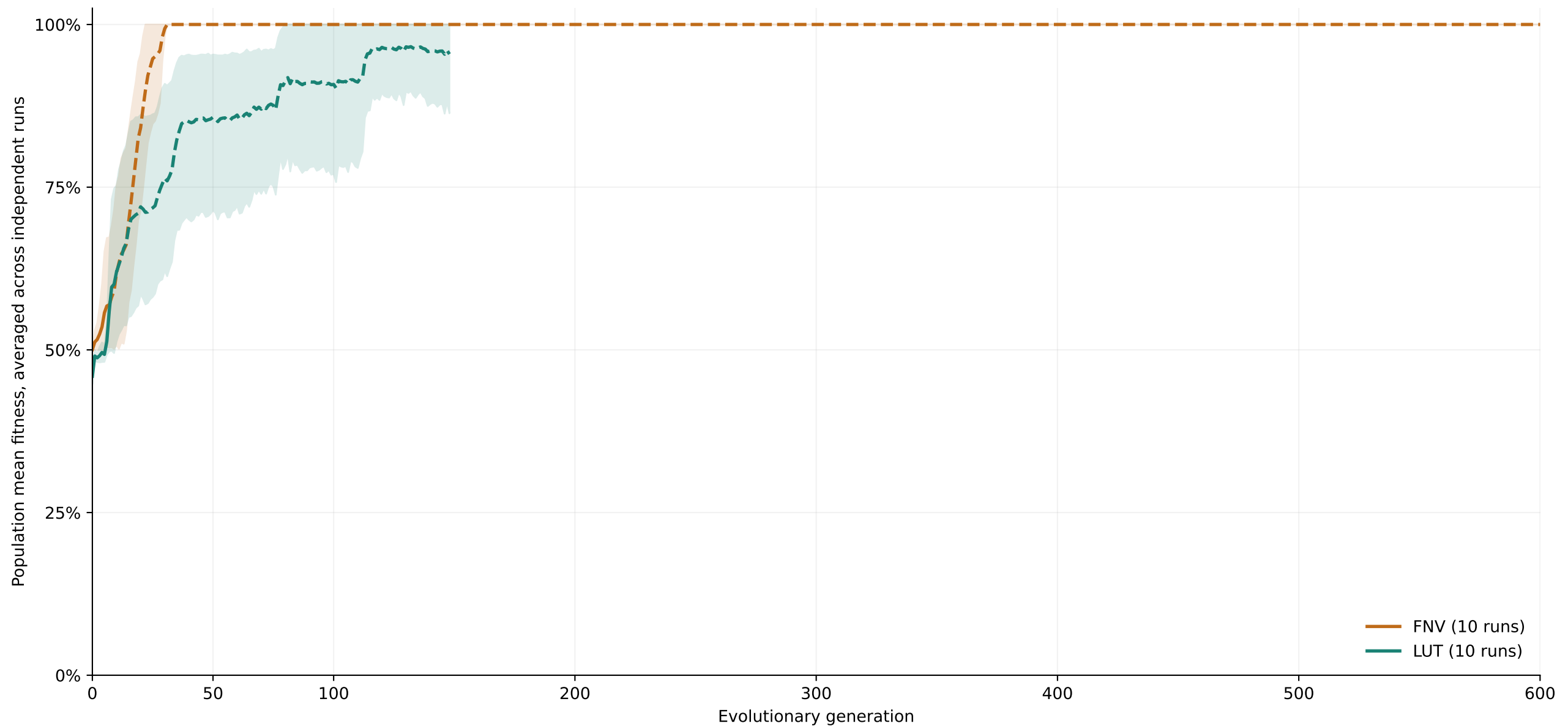
Fig. 43. Parity-3 (XOR3): developmental evolution through generation 600.
