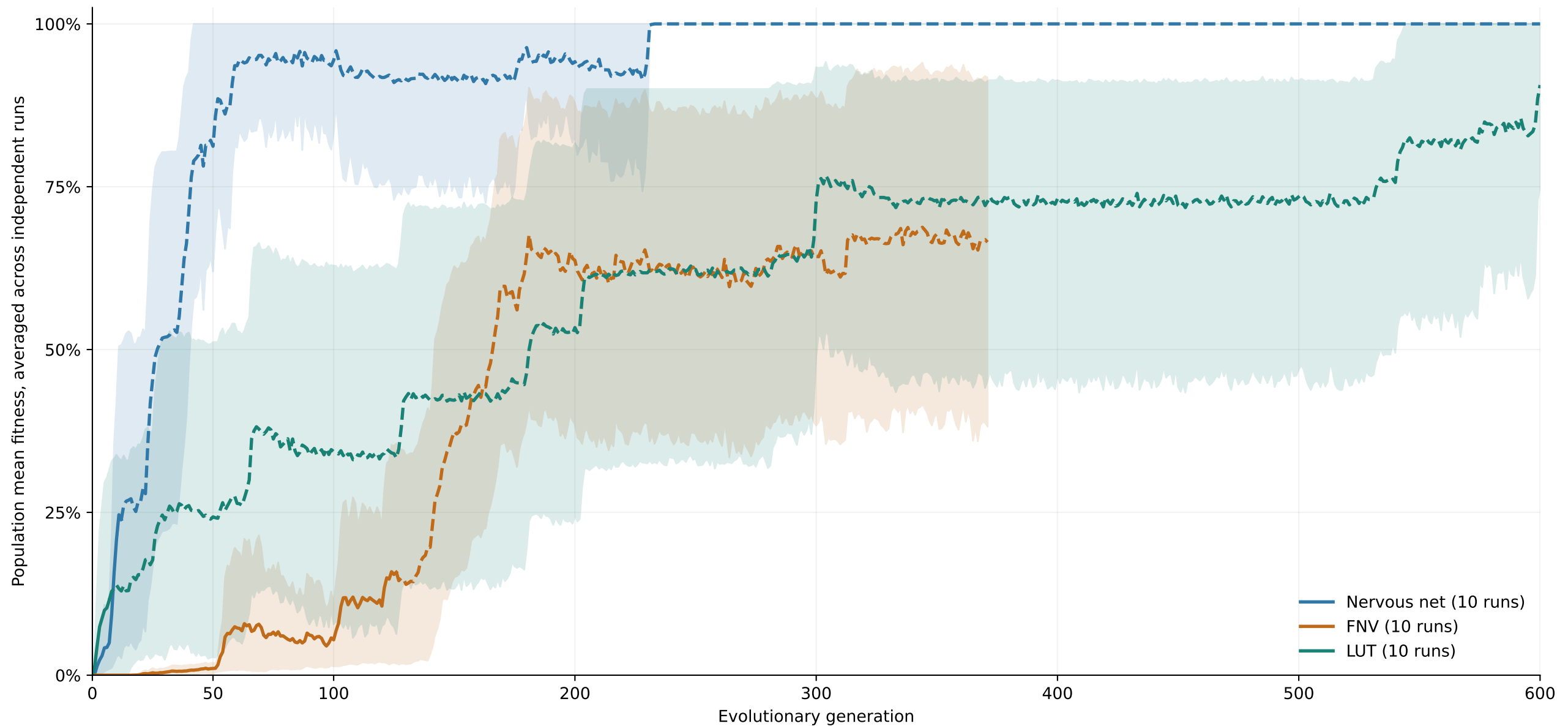
Fig. 45. Pattern (1000): developmental evolution through generation 600.
