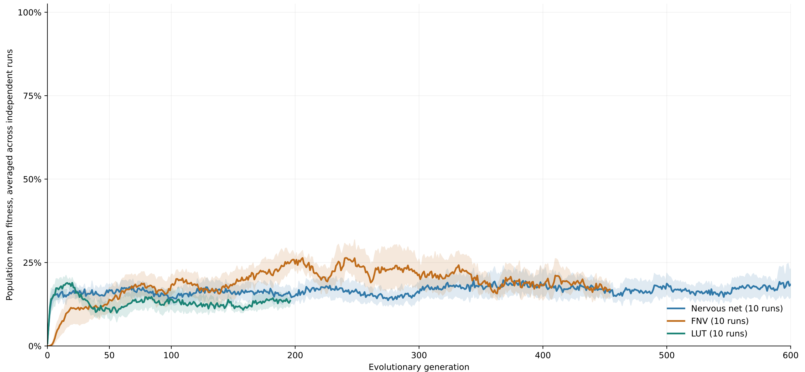
Fig. 51. Resettable divide-by-4: developmental evolution through generation 600.
