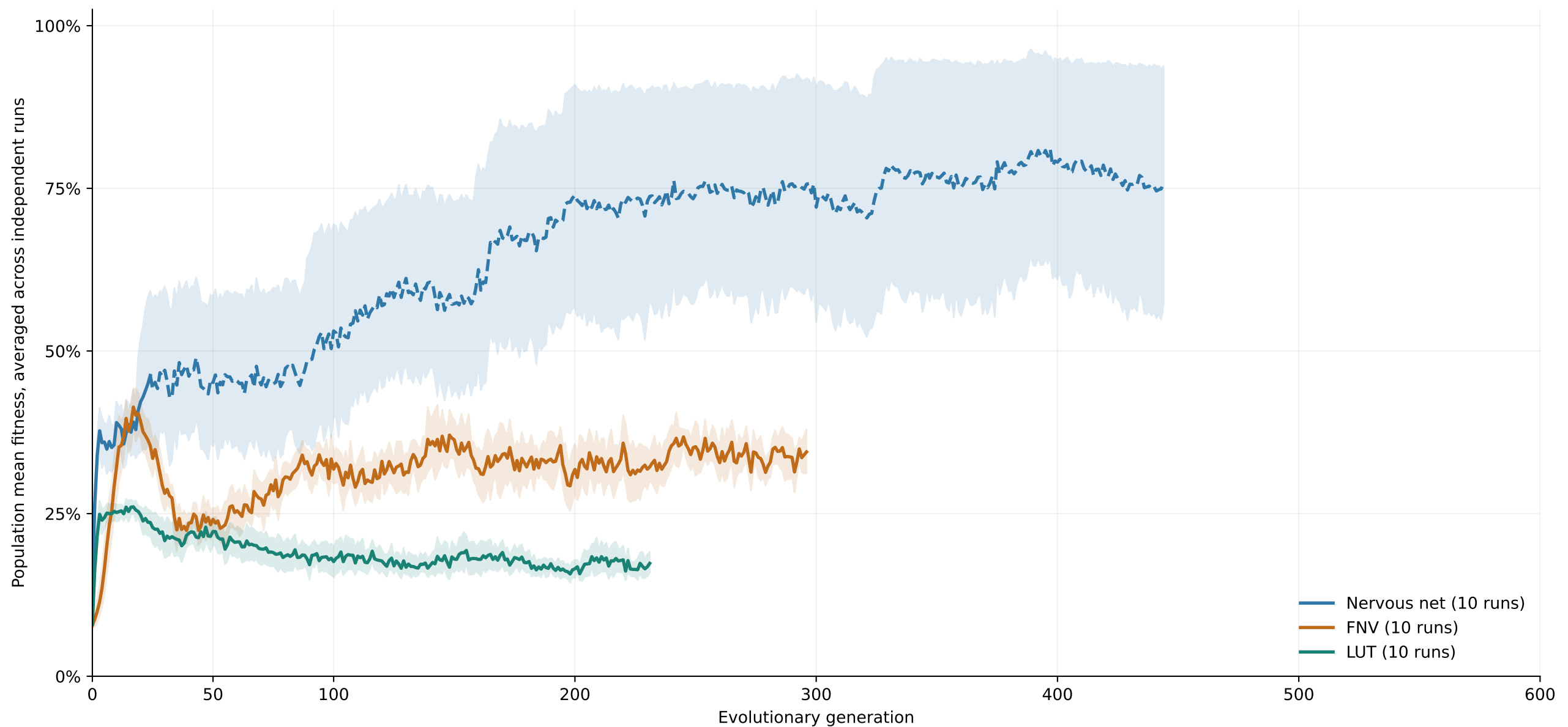
Fig. 52. Resettable toggle: developmental evolution through generation 600.
