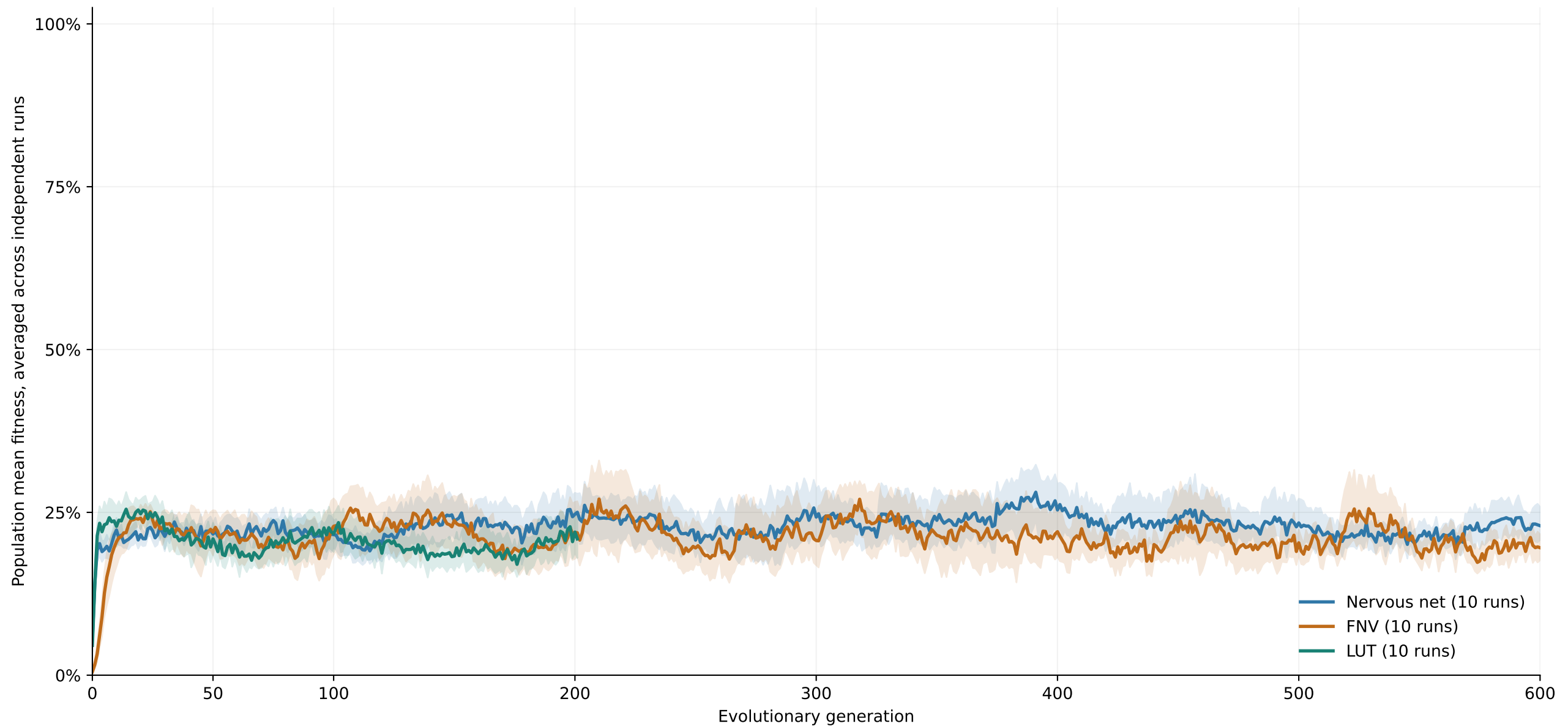
Fig. 58. Temporal sum ( \delta A + \delta B ): developmental evolution through generation 600.
