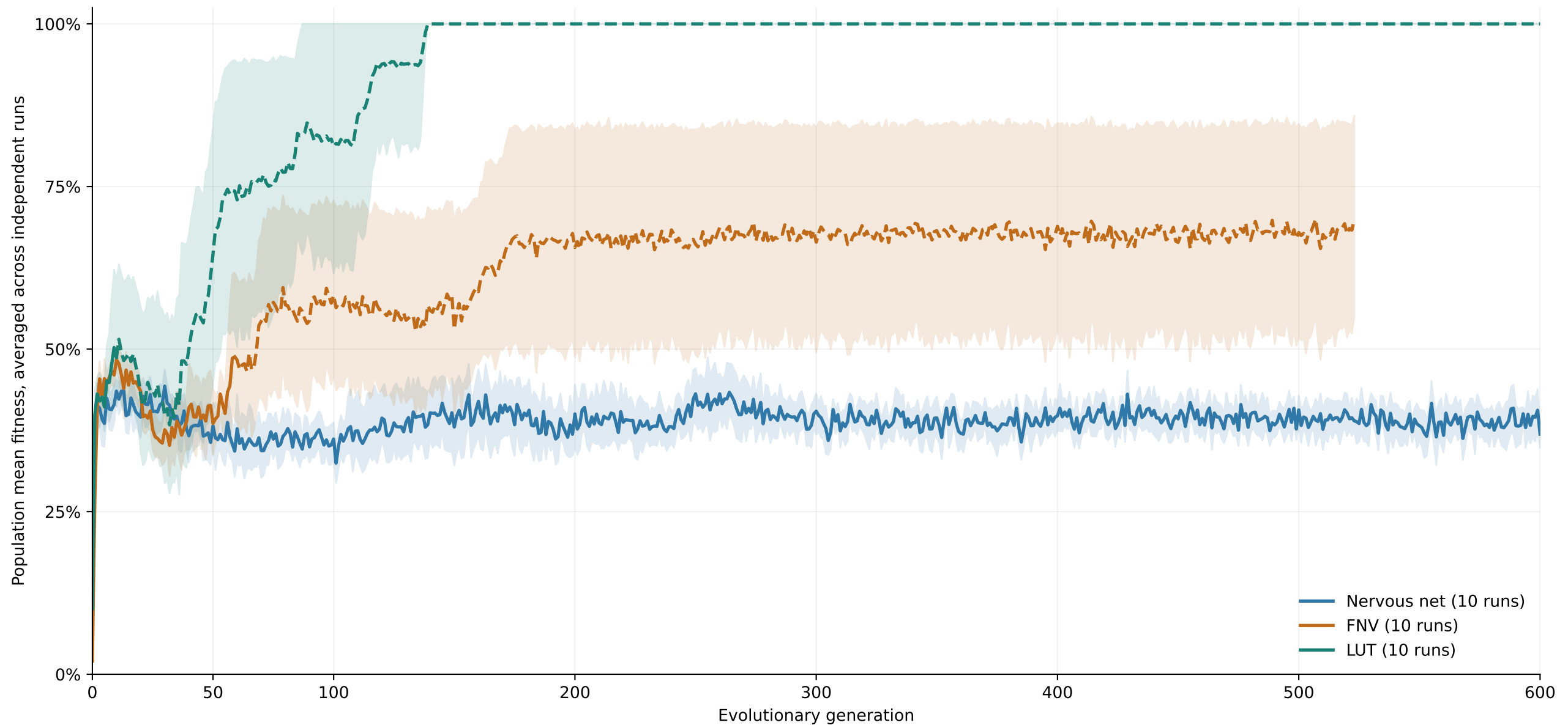
Fig. 62. XNOR (temporal): developmental evolution through generation 600.
