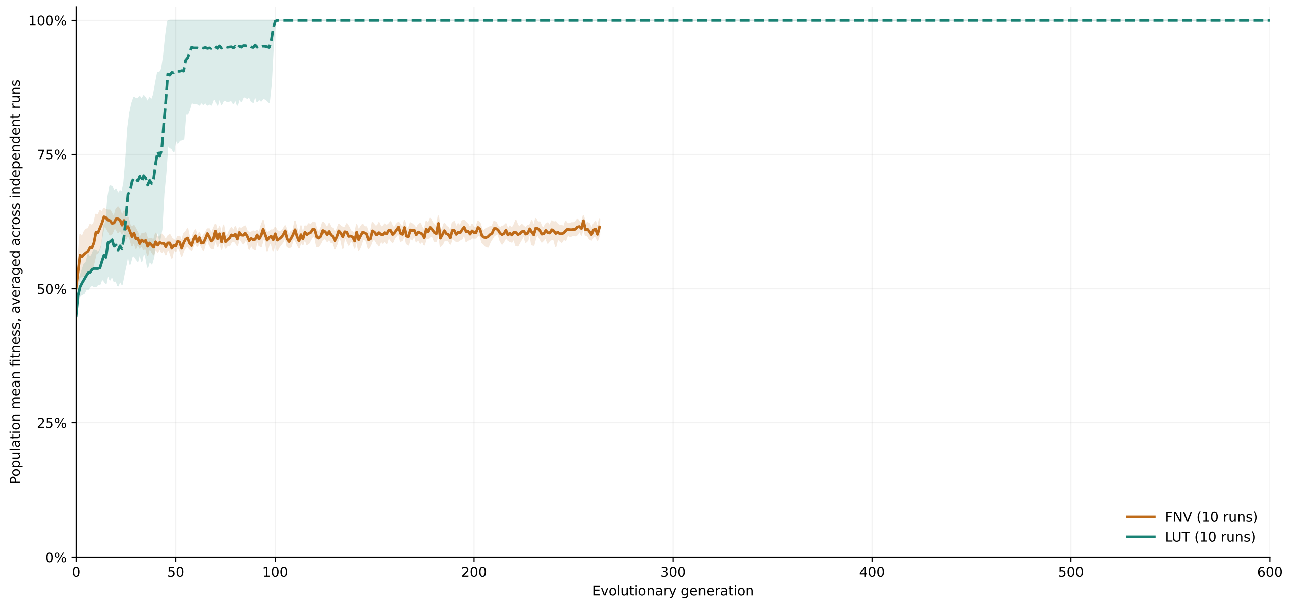
Fig. 61. XNOR: developmental evolution through generation 600.
