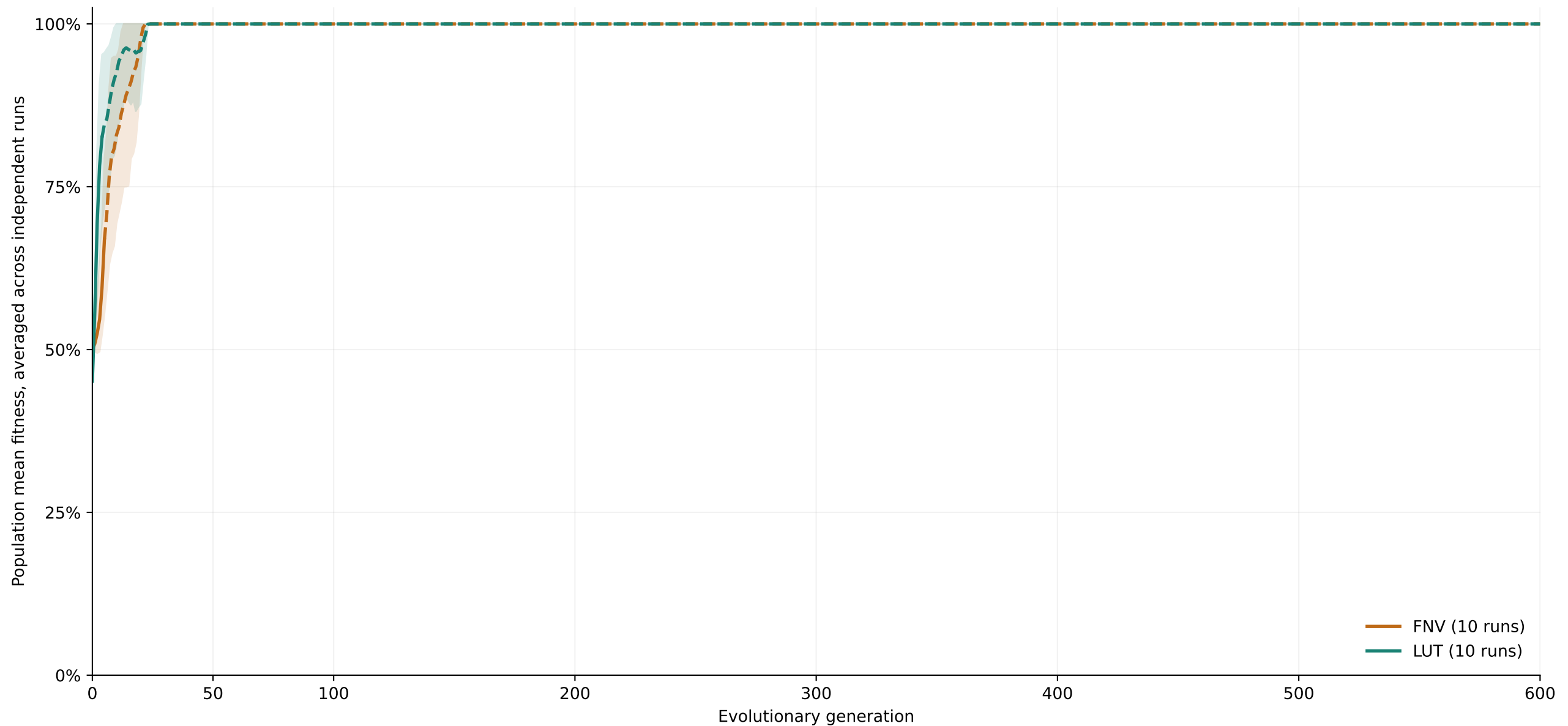
Fig. 63. XOR: developmental evolution through generation 600.
