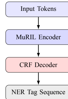
Fig. 1. Baseline MuRIL + CRF architecture for Hindi health-domain NER.
