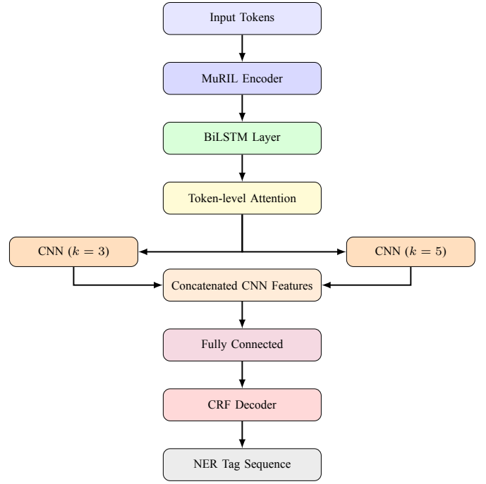
Fig. 2. Stacked MuRIL-based architecture integrating BiLSTM, token-level attention, CNN feature extraction, and CRF decoding for Hindi health-domain NER.
