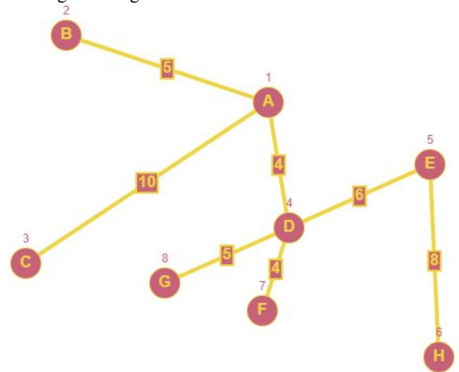
Fig. 3 DFS numbering on the MST
