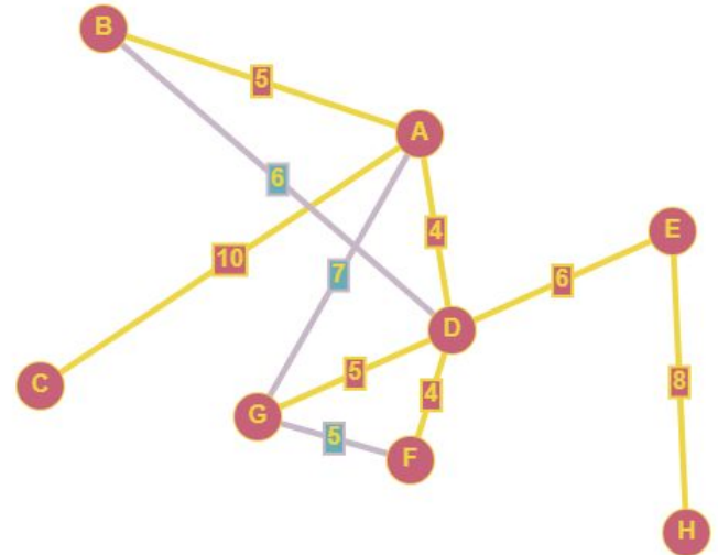
Fig. 2 MST of the graph G
