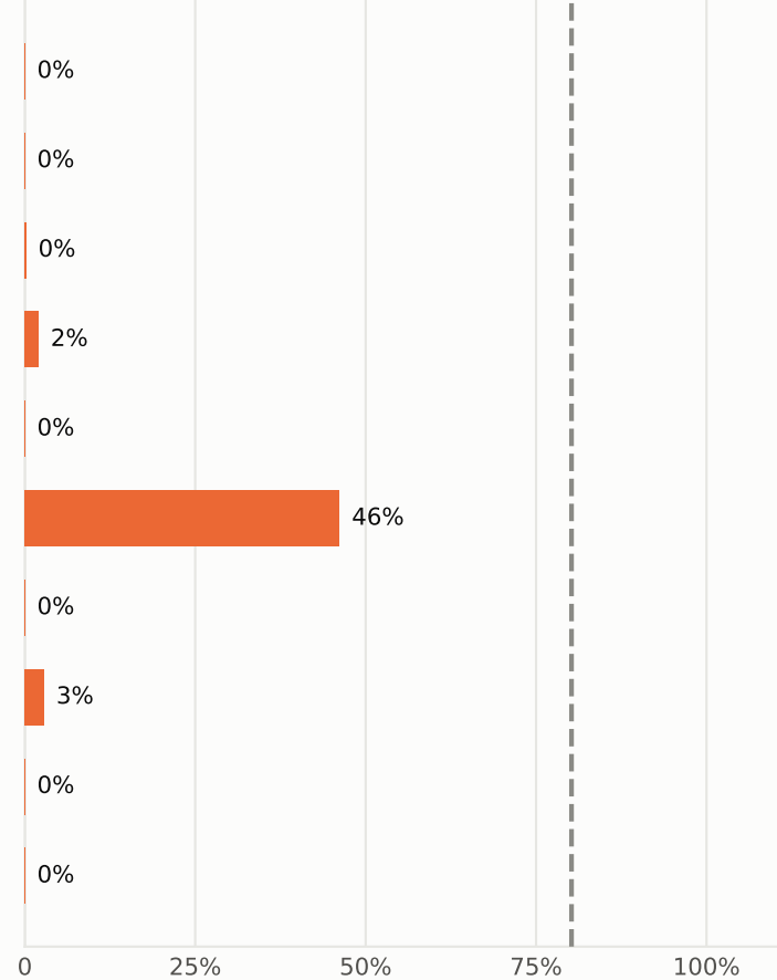
Genome-scale glucose minimal baseline 80%
