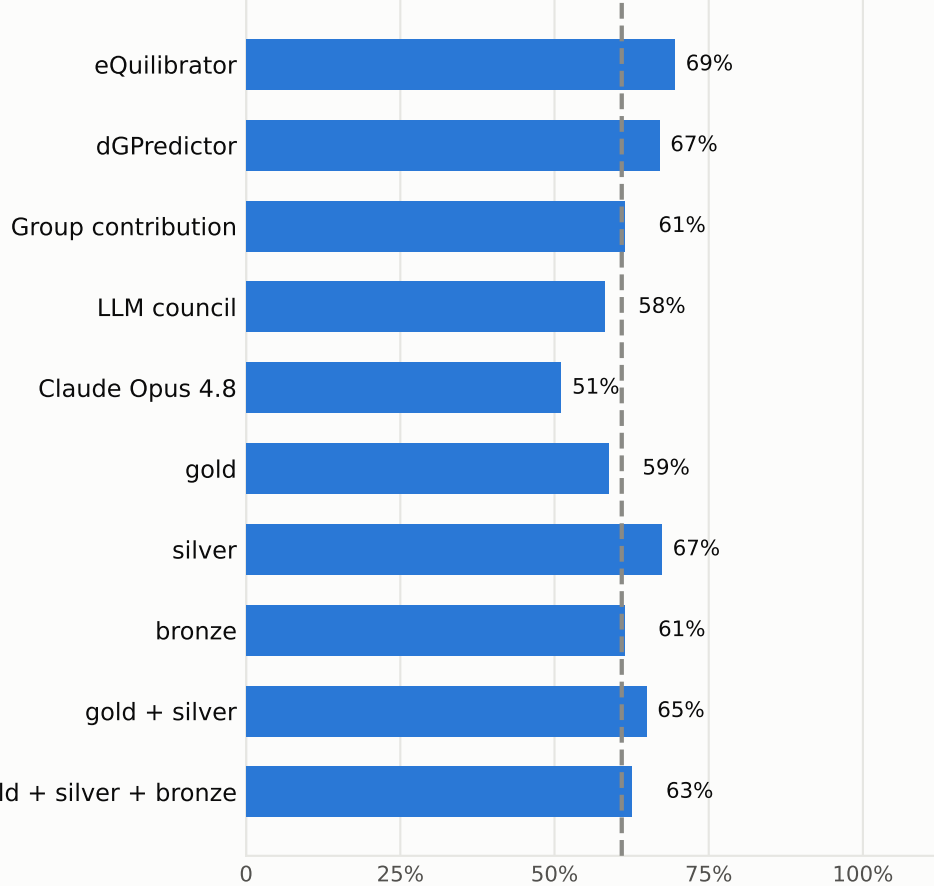
Core models complete media baseline 61%
