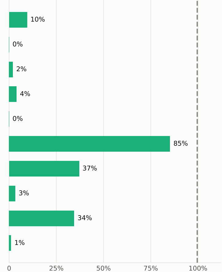
Genome-scale auxotrophy baseline 100%
