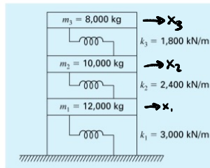
Figure 4: A three-story building modeled as a mass-spring system.
