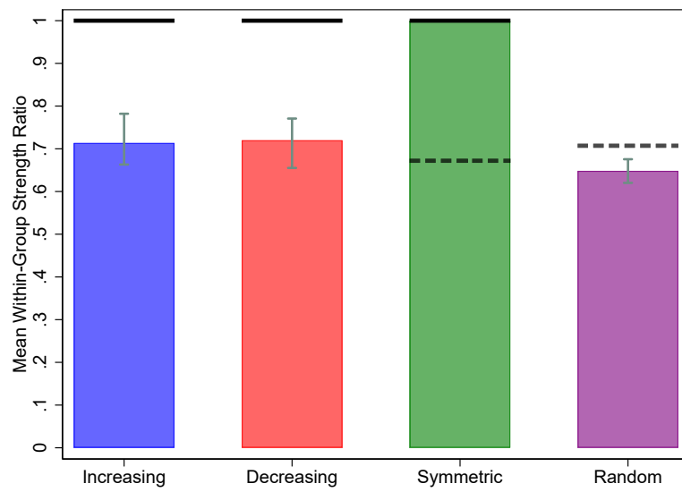
Figure 21: Strength Ratio
