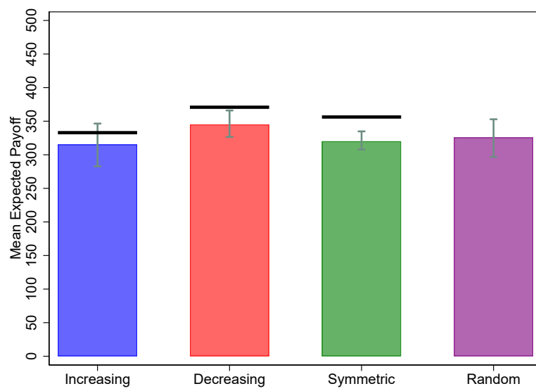
Figure 14: Expected Payoffs
