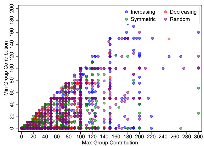
Figure 20: Group Coordination
