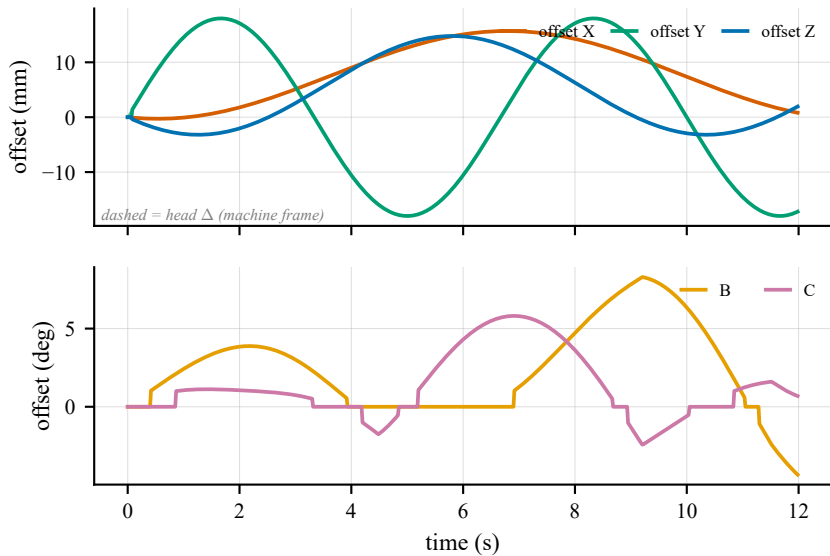
(b) Nozzle offset tracks head motion
