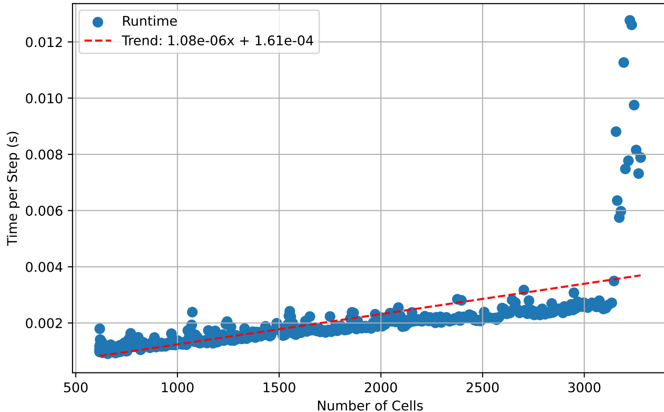
Runtime Scaling with Cell Count
