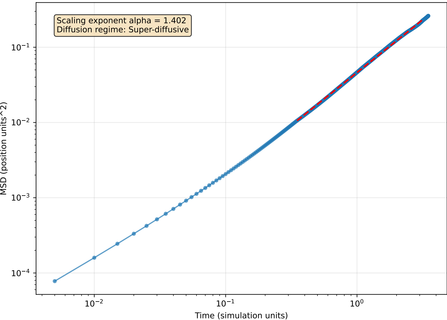
Mean Squared Displacement (N = 479 particles)
