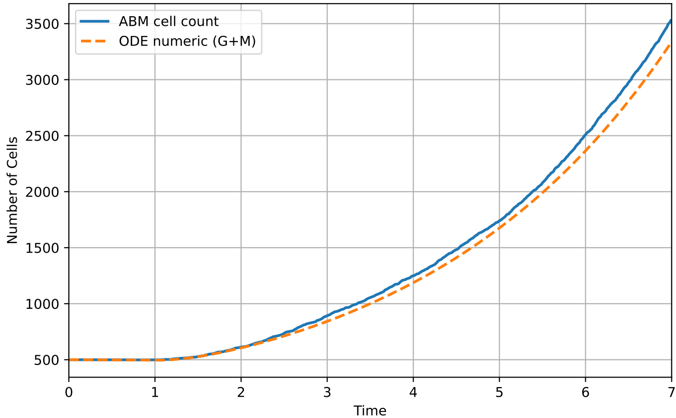
Cell Count vs Time (Numeric ODE)
