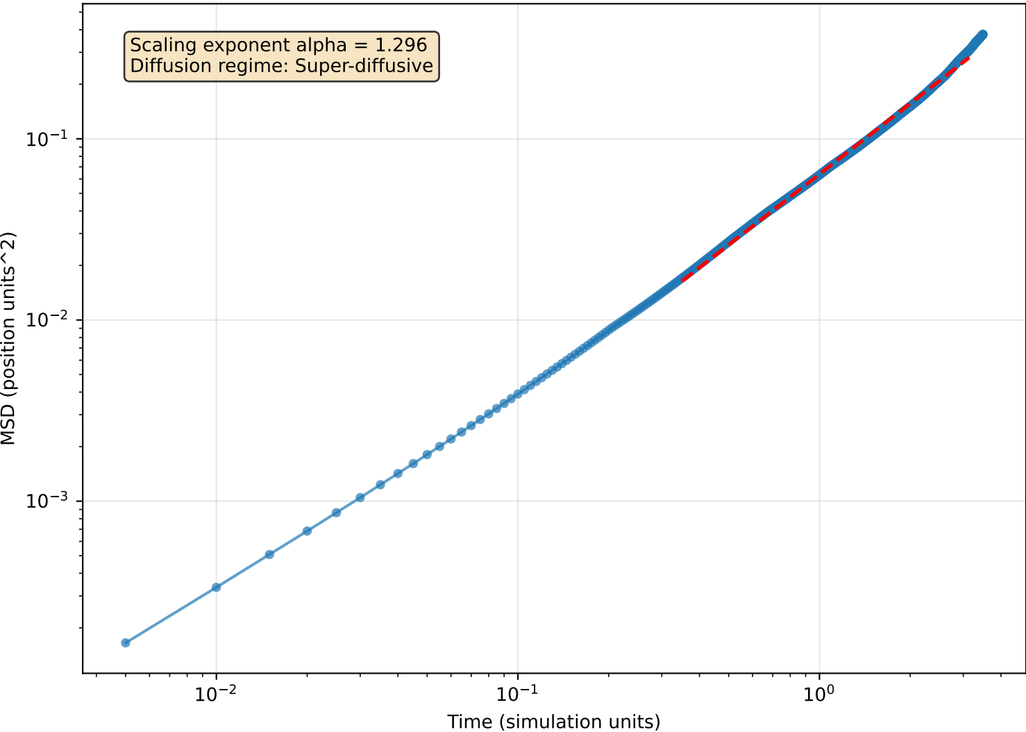
Mean Squared Displacement (N = 490 particles)
