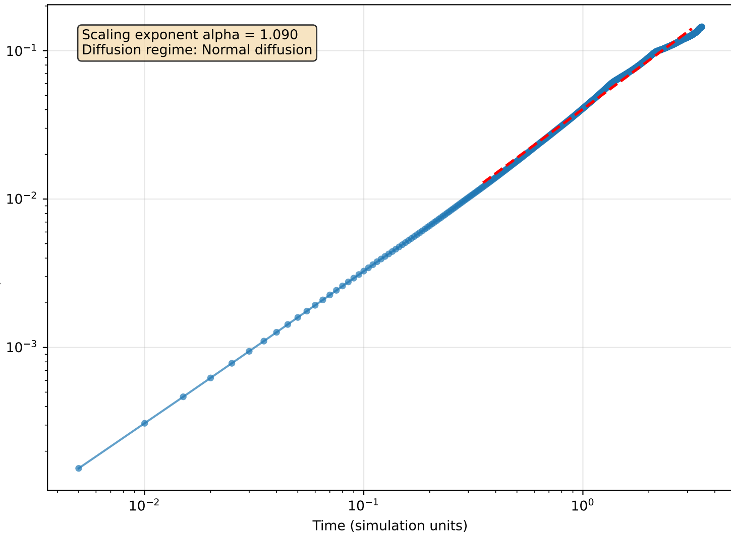
Mean Squared Displacement (N = 486 particles)
