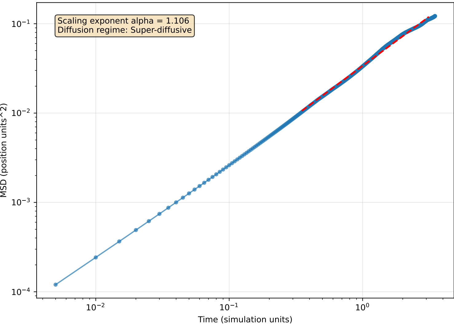
Mean Squared Displacement (N = 488 particles)
