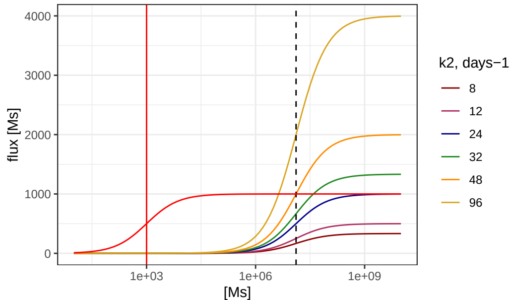
effect of transport rate k_2 on the inhibition of specific IgA flux
