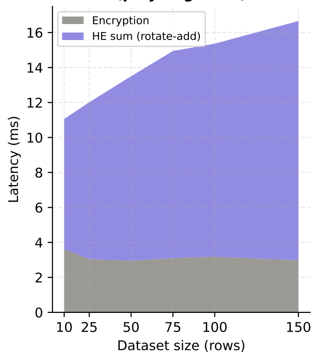
Time breakdown: encrypt vs. sum (poly deg 8192)
