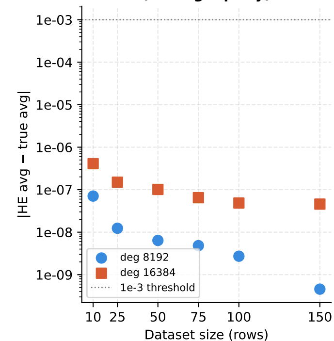
CKKS approximation error (average query)
