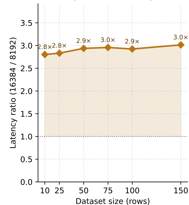
Cost of doubling poly degree (16384 vs. 8192)
