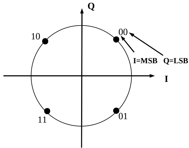
Figure 2.4.10-2: Constellation Mapping
