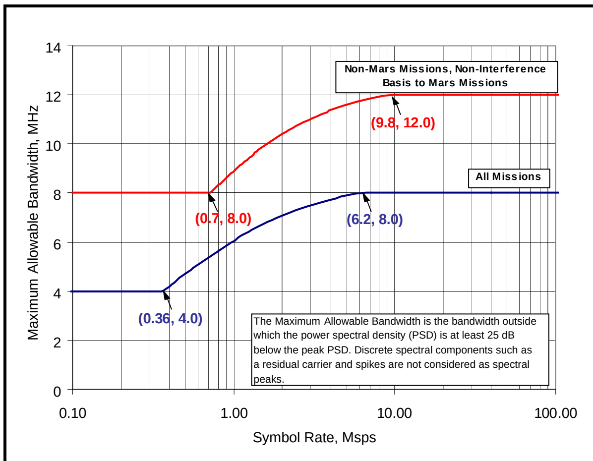
Figure 3.1.2B-1: Maximum Allowable Bandwidth (B25) vs. Symbol Rate (Rs) (in the Transition Regions, B_{25} \text{ in MHz} = k \cdot R_s / (0.41 + R_s) where k = 8.53 and 12.5 for All-Missions and Non-Mars Missions, Respectively)
