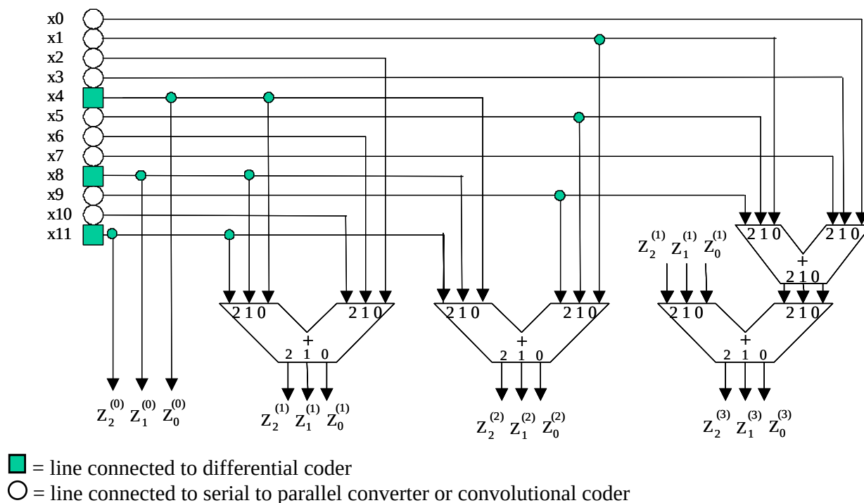
Figure 2.4.18-8: Constellation Mapper for 2.75 Bits/Channel-Symbol
