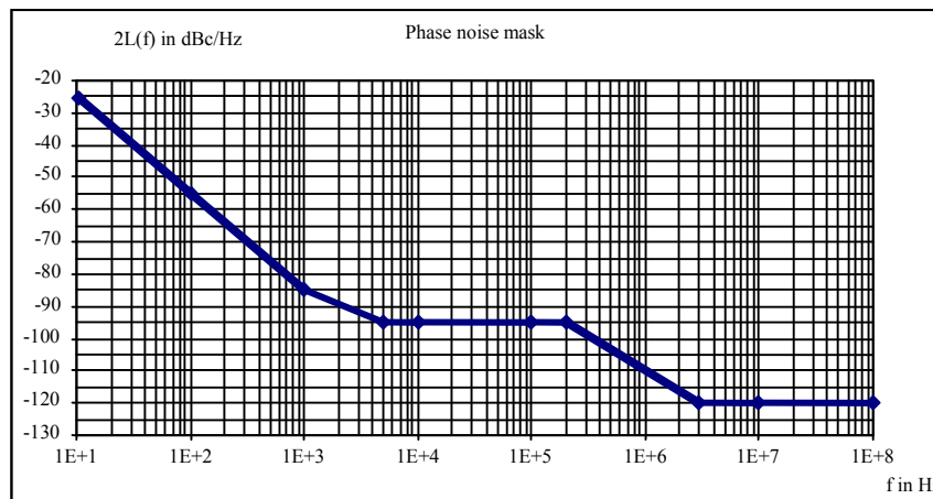
Figure 2.4.18-13: 8PSK Phase Noise Mask Recommendation
