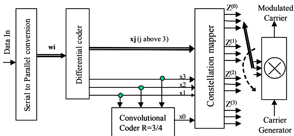
Figure 2.4.18-2: Structure of the 4D 8PSK-TCM Code/Mapper
