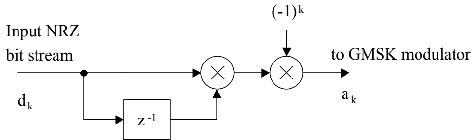
Figure 2.4.18-1: GMSK Precoder
