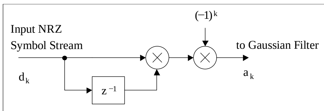
Figure 2.4.22A-2: GMSK Precoder
