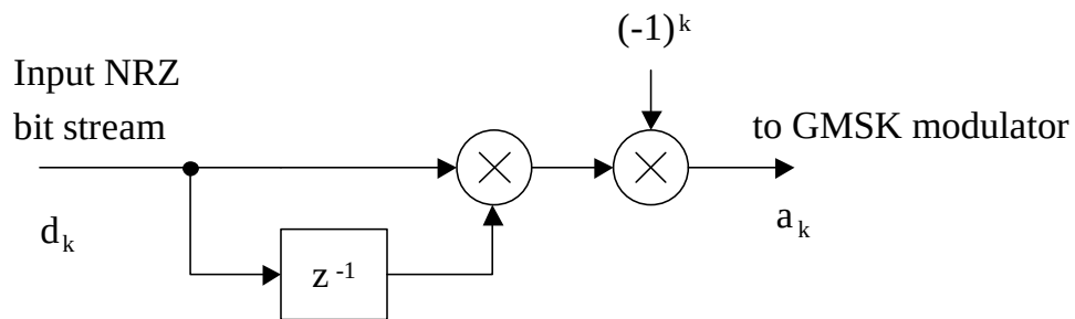
Figure 2.4.17B-1: GMSK Precoder
