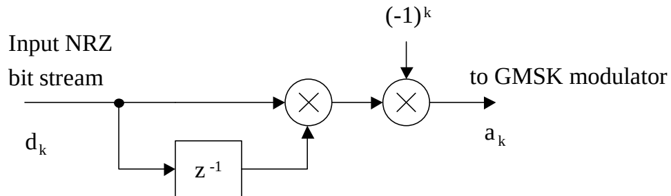
Figure 2.4.20B-1: GMSK Precoder
