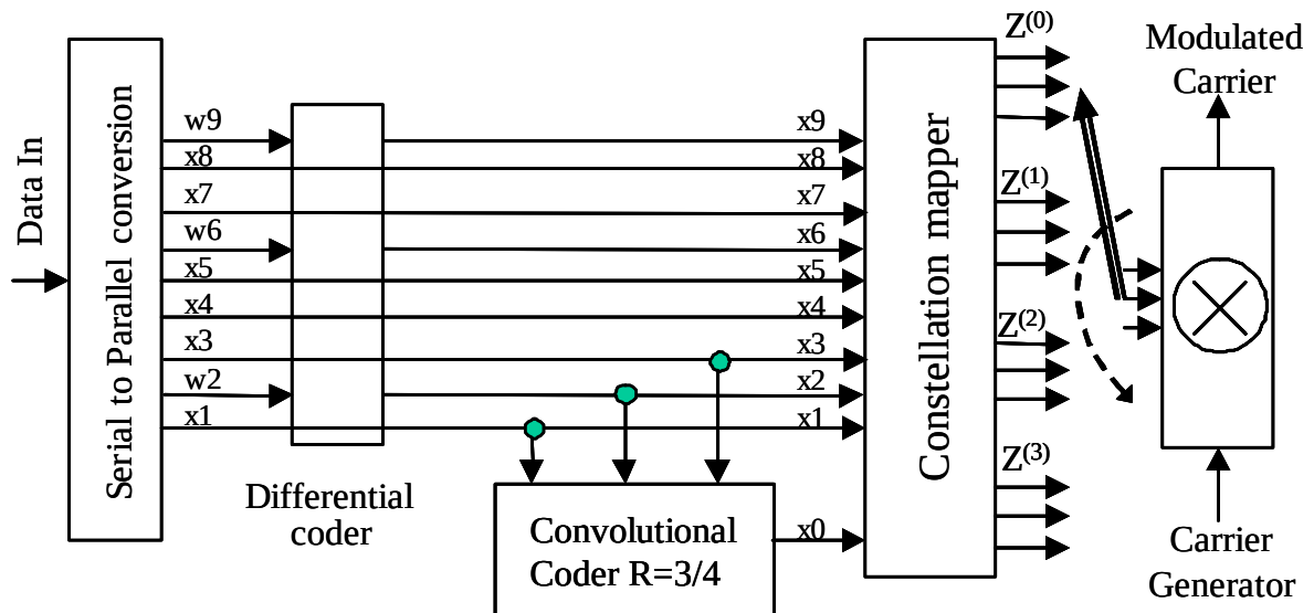
Figure 2.4.18-9: Coder and Mapper Implementation at 2.25 Bits/Channel-Symbol Efficiency
