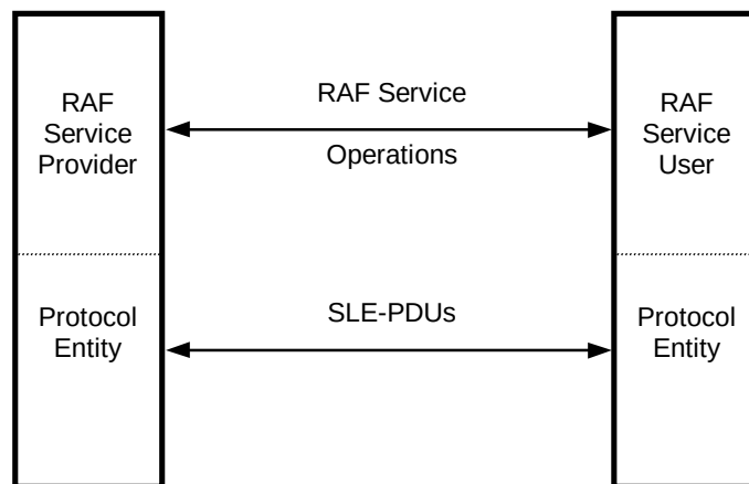
Figure 2-5: Mapping of RAF Service Operations to SLE-PDUs
