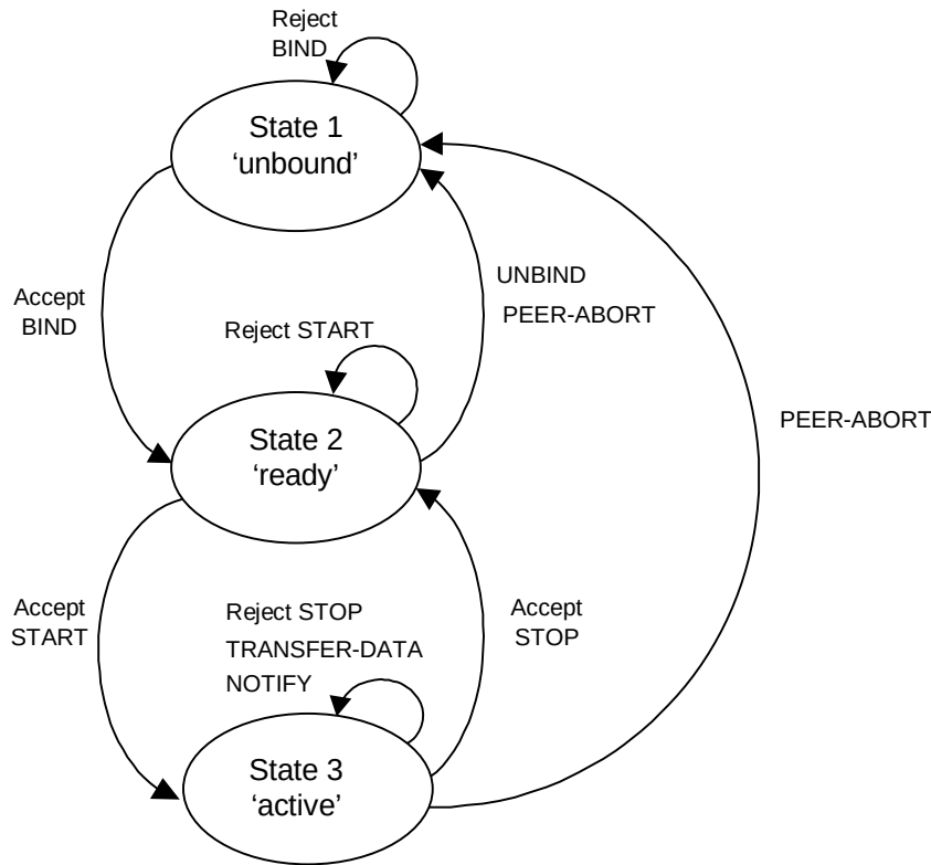
Figure 2-4: Simplified RAF Service Provider State Transition Diagram
