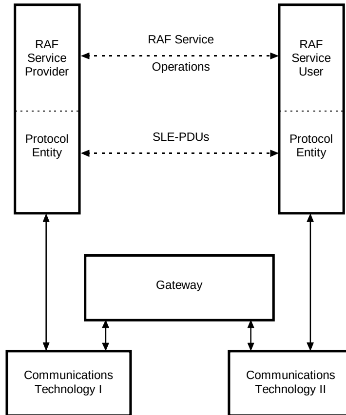
Figure 2-6: RAF Service Provision Via a Gateway
