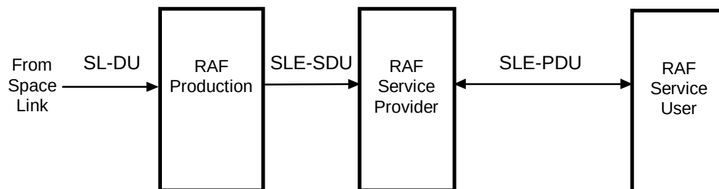
Figure 2-2: RAF Service Production and Provision
