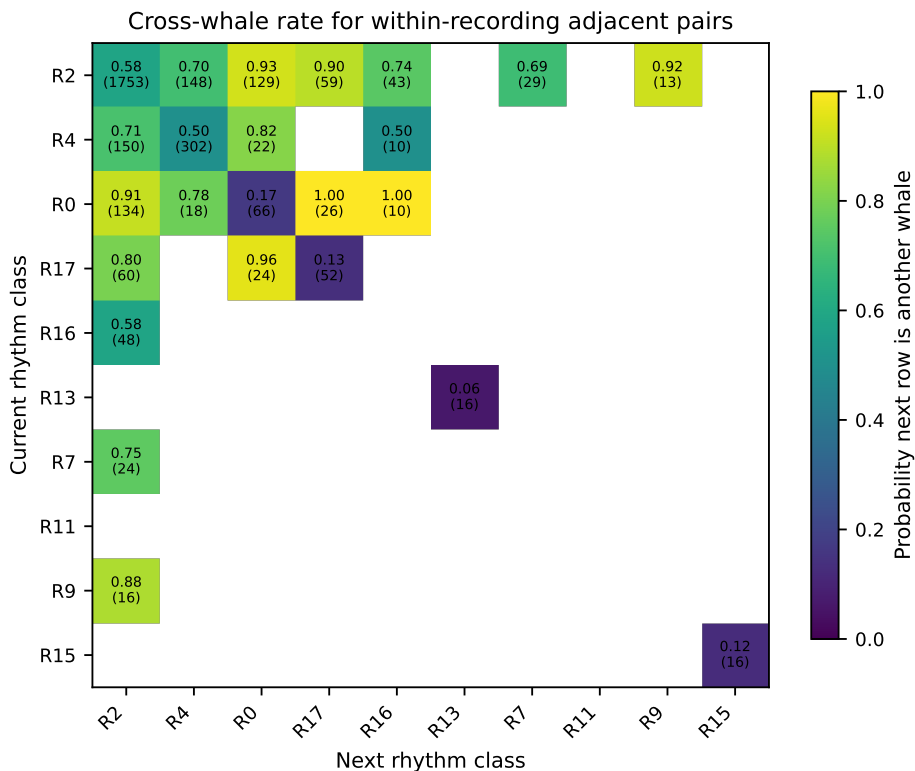
Figure 4: Cross-whale rate for selected same-REC adjacent rhythm pairs. Numbers in cells show rate and count. High R0–R2 and R17–R0 rates motivate handoff and escalation glosses.
