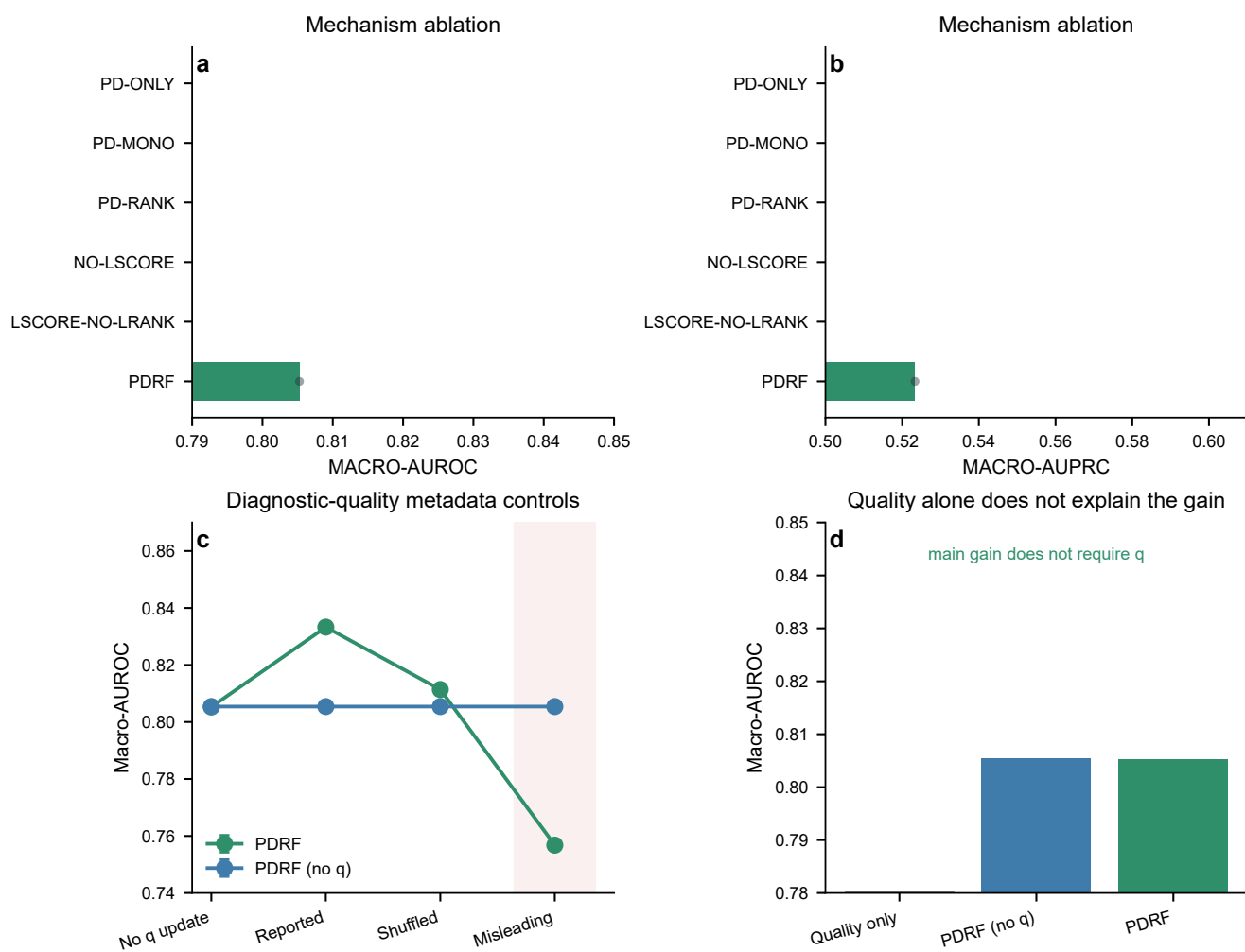
Figure S10: Original-protocol mechanism and diagnostic-quality controls. Mechanism ablations, metadata perturbations and a quality-only comparator are retained as sensitivity evidence.
