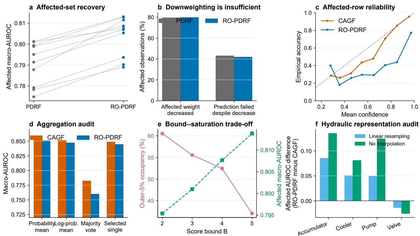
Figure S13: Prediction-level recovery and deployment audits. Matched recovery, failures despite downweighting, affected-row calibration, aggregation rules, score-bound sensitivity and hydraulic representation robustness.
