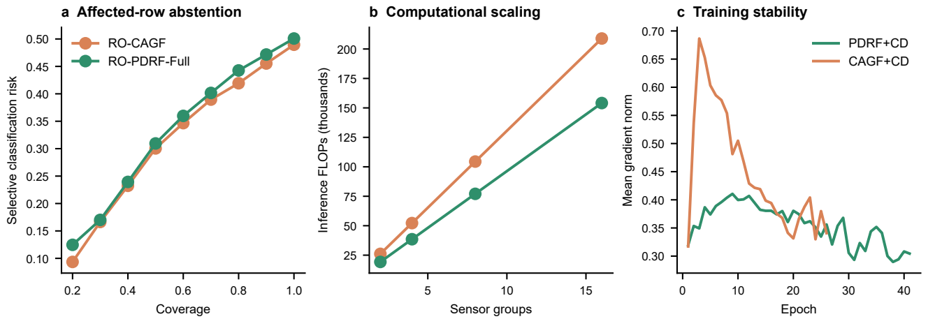
Figure S9: Deployment and optimization audits. a , affected-row selective classification risk. b , counted inference FLOPs versus sensor-group count. c , mean pre-clipping gradient norm by epoch for the two clean-distillation controls.
