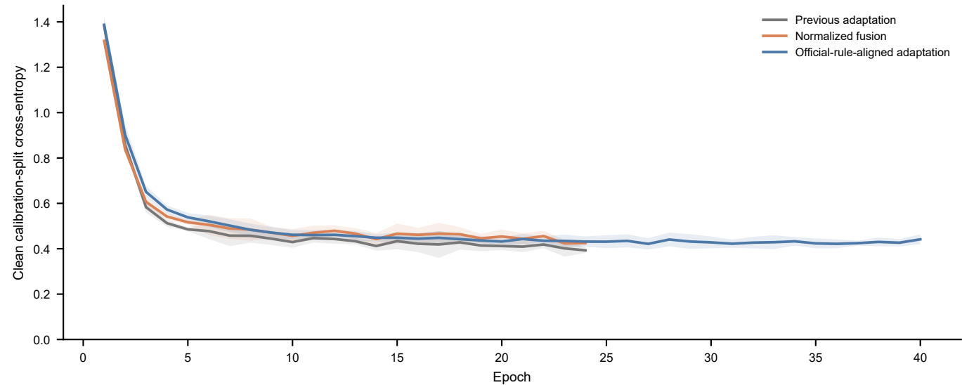
QMF sensor-group adaptation training audit
