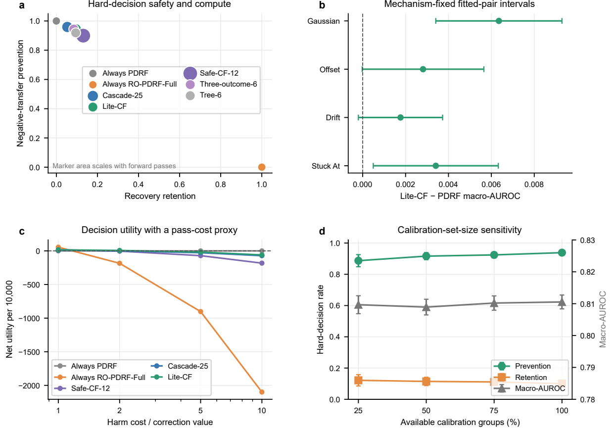
Figure 3: Hard-decision safety, uncertainty and compute. a , negative-transfer prevention versus recovery retention on the strict subset; marker area scales with mean forward passes, and the always-endpoint rows define the two corners. b , Lite-CF minus PDRF macro-AUROC with each fault mechanism held fixed; bars are paired 95% Student- t intervals across 10 fitted model pairs. c , net utility per 10,000 strict observations as the cost of one realized harm increases relative to the value of one retained correction; the plotted pass penalty is a forward-pass/FLOP proxy, not measured energy. d , repeated calibration-group subsampling; bars show 95% intervals over seed-repeat summaries.
