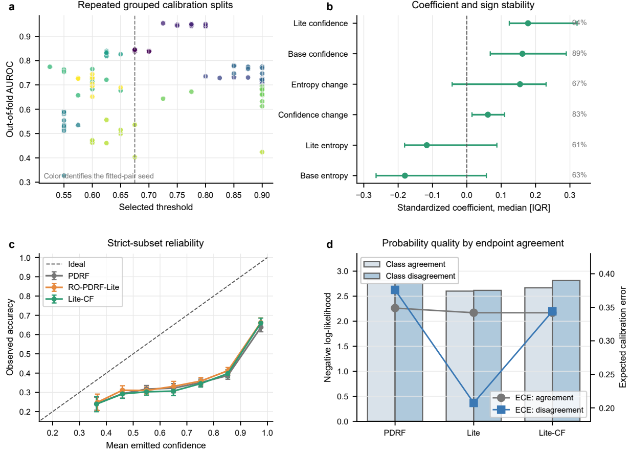
Figure 4: Selector stability and final probability quality. a , selected threshold and out-of-fold preference AUROC across 100 repeated grouped fits; colour identifies the fitted endpoint-pair seed and the dashed line marks the overall median threshold. b , median standardized Lite-CF coefficient with interquartile range; right-side percentages are dominant-sign frequencies. c , reliability curves for temperature-scaled strict-subset outputs; points aggregate fault-seed cells within confidence bins. d , negative log-likelihood bars and 15-bin expected calibration error lines after separating cases on which the endpoint classes agree or disagree.
