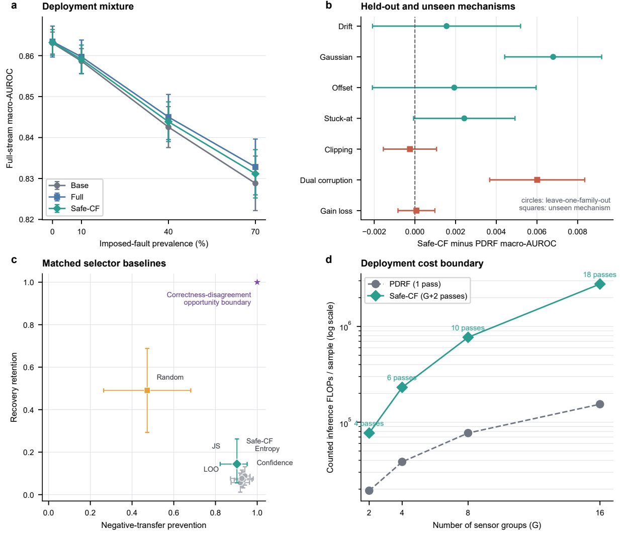
Figure 3: Cross-fitted selective recovery under deployment and transfer audits. a , complete held-out streams as imposed-fault prevalence increases; the 0% point contains exactly one clean value per seed, nonzero points first average mechanisms within seed, and bars are seed-level 95% Student- t intervals. b , Safe-CF minus PDRF macro-AUROC under leave-one-family-out and unseen-mechanism audits; bars are paired seed-level 95% Student- t intervals. c , negative-transfer prevention versus recovery retention for cross-fitted, simple and random selectors; Safe-CF bars are crossed-cluster 95% bootstrap intervals and other bars are seed-level 95% Student- t intervals. The star marks the correctness-disagreement opportunity boundary. d , counted linear-layer FLOPs for PDRF and Safe-CF as the number of sensor groups increases; Safe-CF requires G + 2 forward passes.
