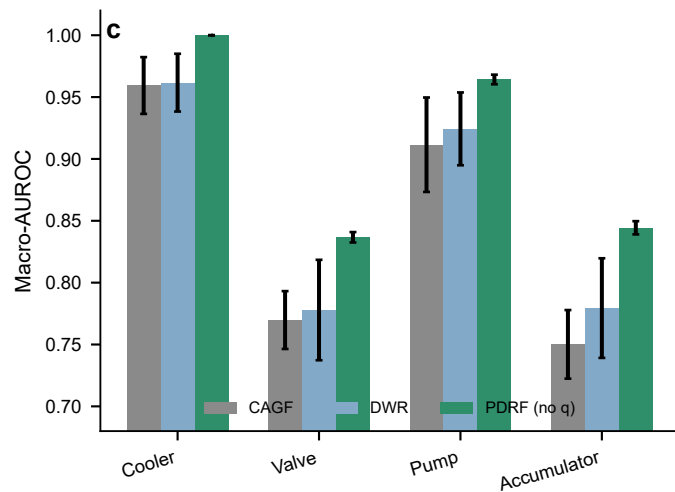
Hydraulic pressure-group fault
