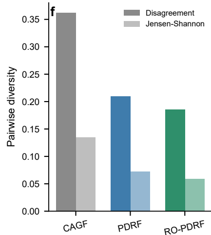
Ensemble diversity audit
