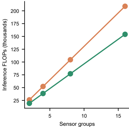
b Computational scaling
