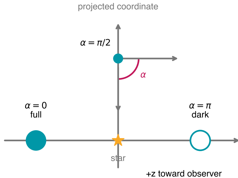
(a) Illumination is a planet-centered angle
