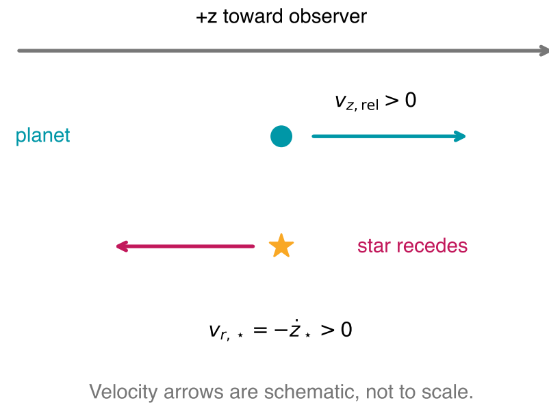
(c) Recession fixes the stellar RV sign
