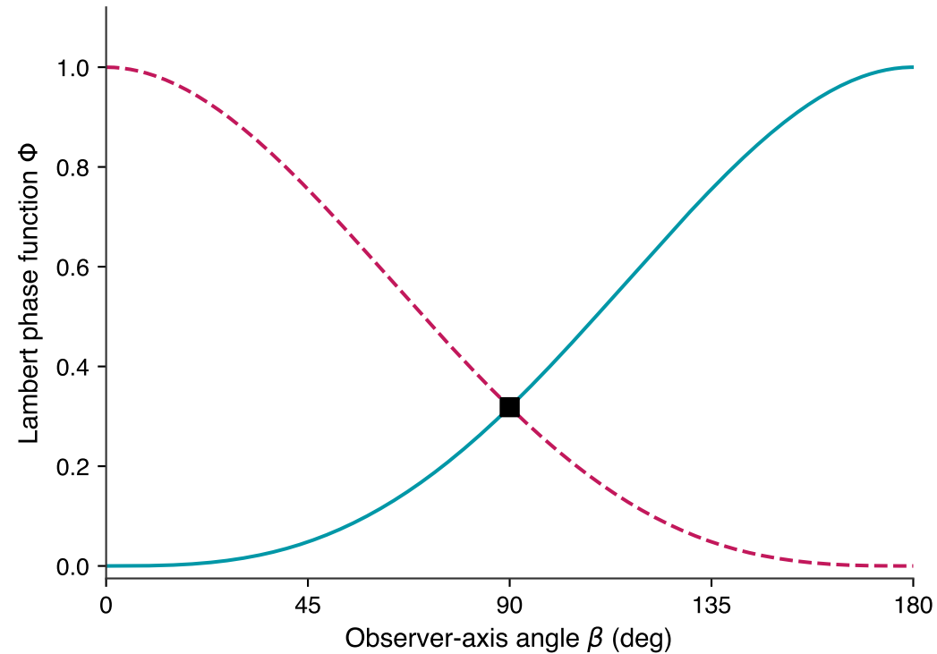
(b) Quadrature hides the error
