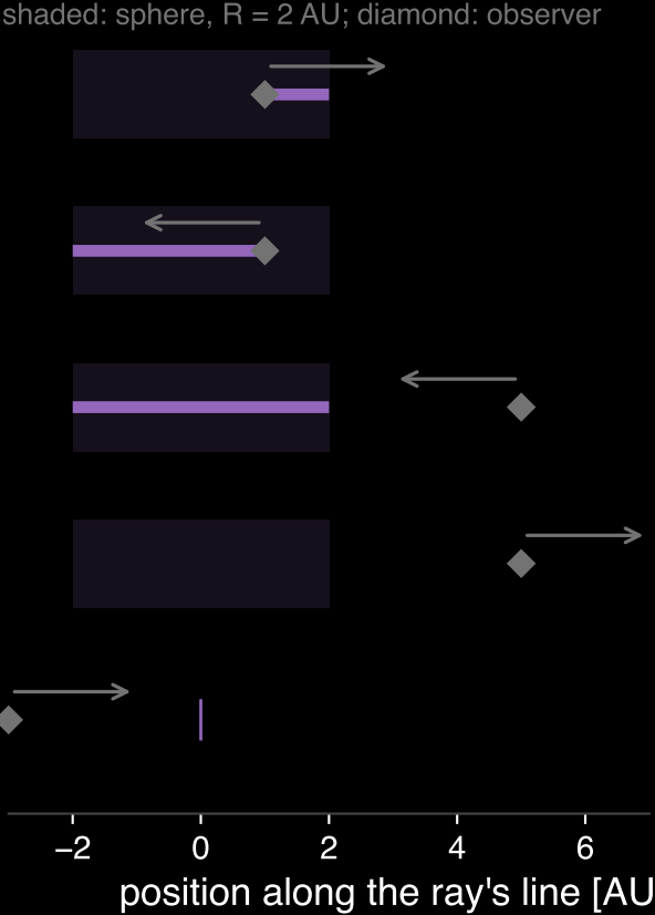
(a) Only the half-ray s \geq 0 is integrated
