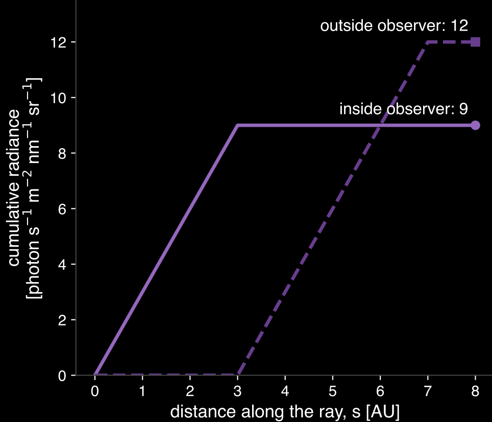
(c) Radiance accumulates only inside the cloud
