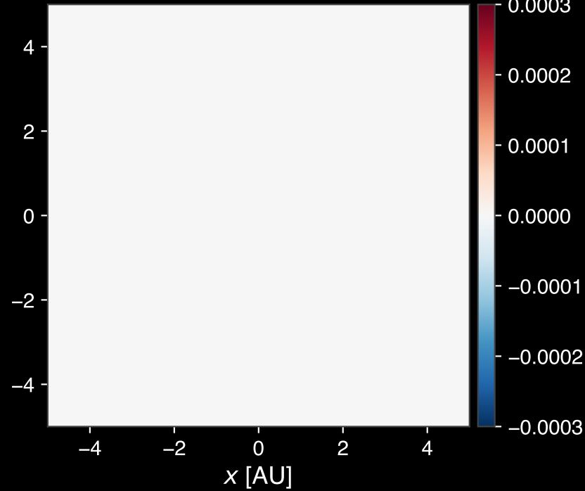
(c) (a) minus (b): \max |\text{diff}| = 0
