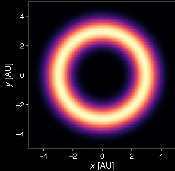
(a) n_{\text{zodis}} = 2 , albedo = 0.15
