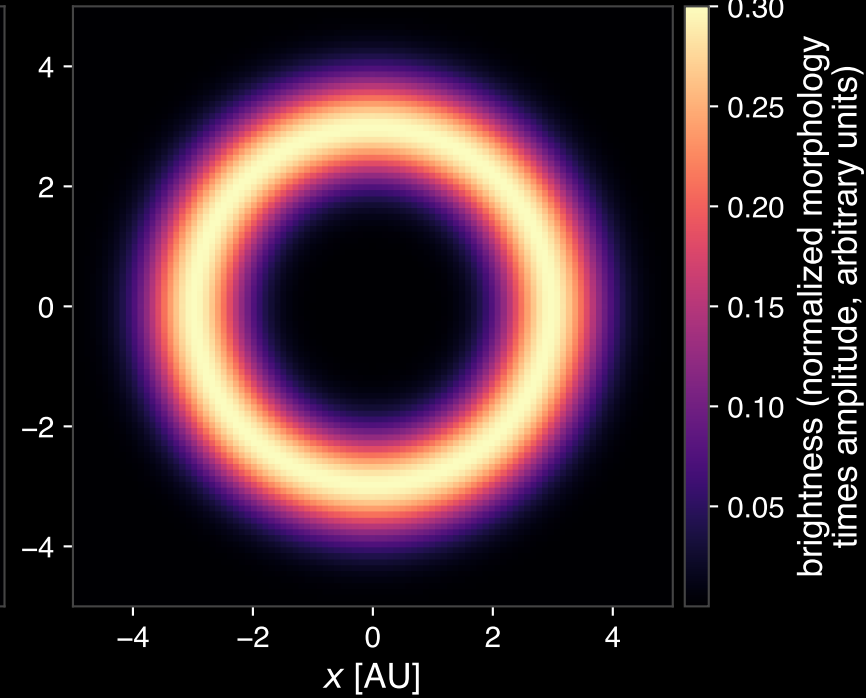
(b) n_{\text{zodis}} = 1 , albedo = 0.3
