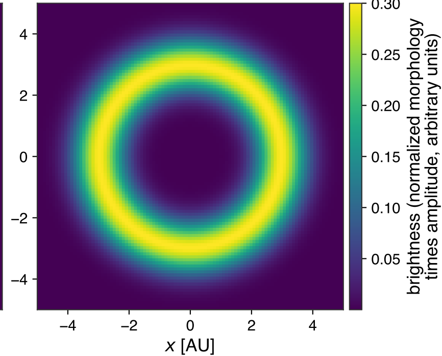
(b) nzodis = 1, albedo = 0.3
