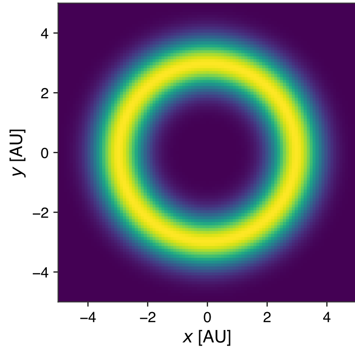
(a) nzodis = 2, albedo = 0.15
