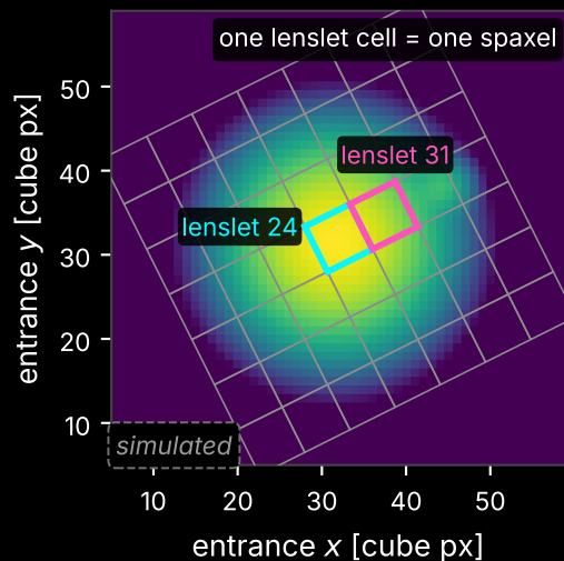
(b) entrance plane: lenslet cells
