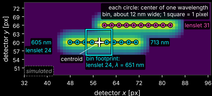
(c) detector: one trace per lenslet
