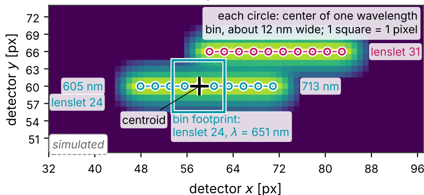
(c) detector: one trace per lenslet
