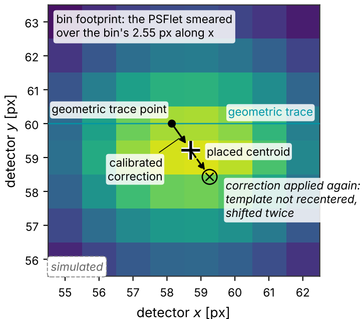
(b) placed on the detector
